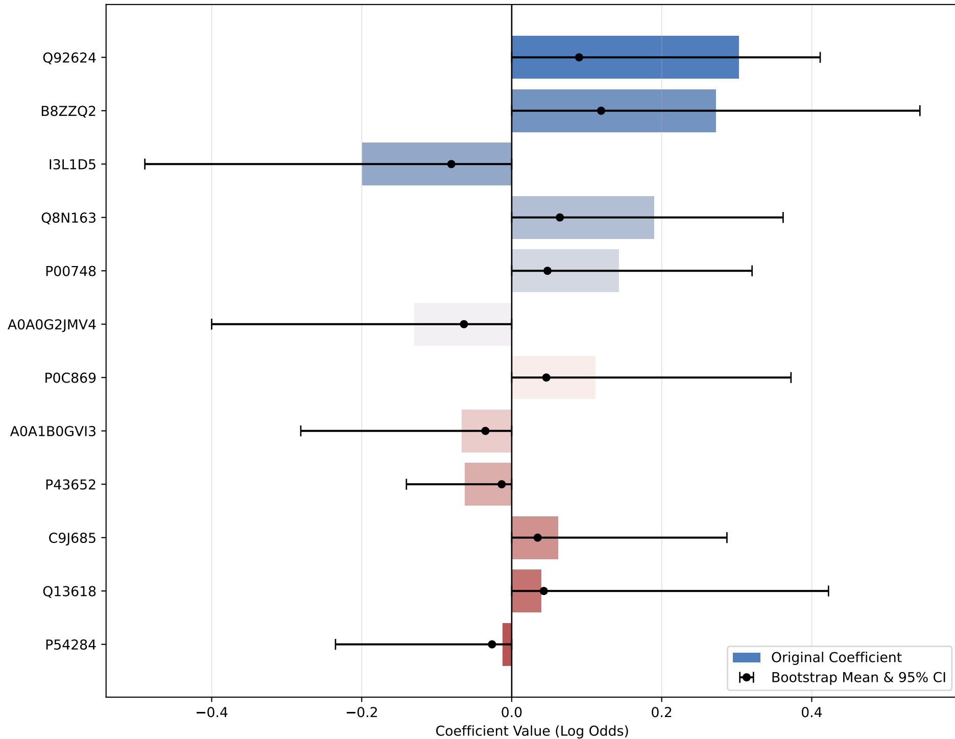
Top 12 Features (Bars = Original, Points/Lines = Bootstrap 95% CI)
